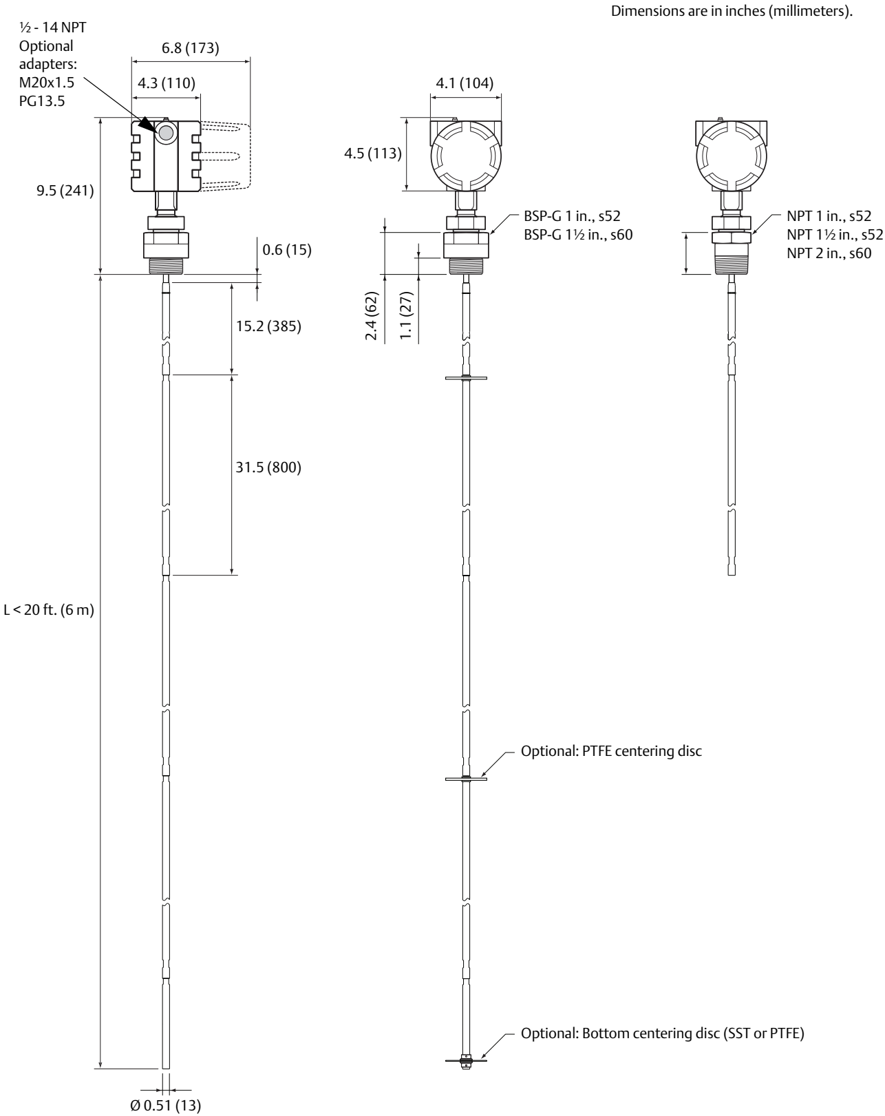
Figure 2. Segmented Rigid Single Lead with Threaded Connection
