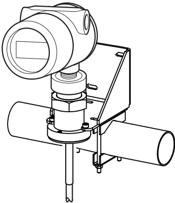
Pipe mounting (horizontal pipe)
