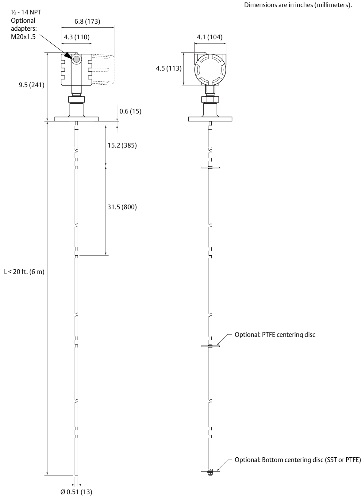
Figure 3. Segmented Rigid Single Lead with Flange Connection
