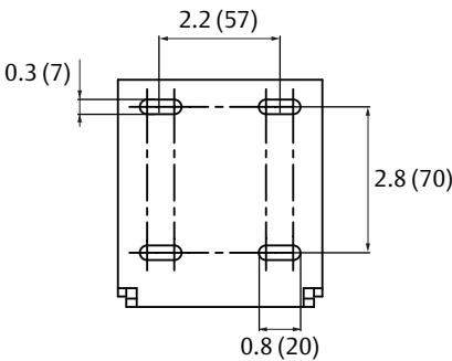
Hole pattern wall mounting
